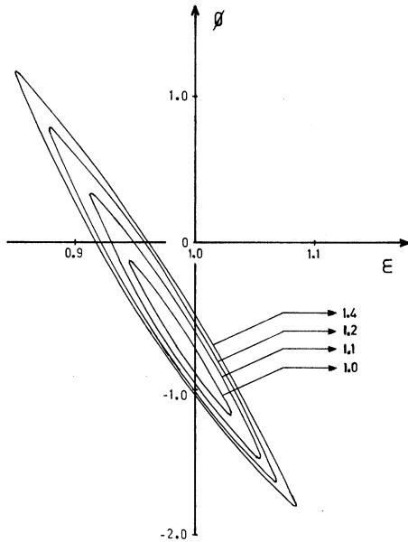
FIG. 3. Contours for the least-squares residual (relative values only) obtained by fitting the form V(r_{hkl})/V_1 \sim A \cos(4.911_0 \epsilon r_{hkl} + \phi)/(r_{hkl})^3 , where \epsilon = (e/at.)^{1/3} , to the pair-interaction ratios obtained from the five sets of data at T/T_c = 1.091 (see Table II). The results are for A = 1.9 .
