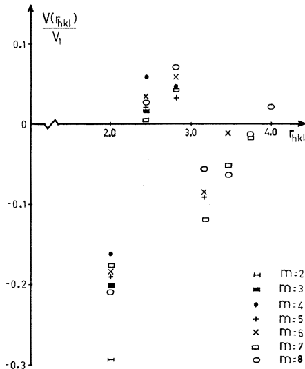
FIG. 2. Variation of the pair-interaction ratios with m , the number of interactions included in the determination. The results were obtained from the \alpha_i data of Moss at T/T_c=1.091 .
