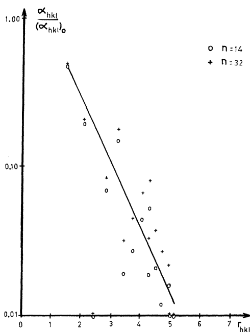
FIG. 1. Comparison of the first fourteen \alpha_i (as functions of distance in the lattice) obtained in the mean-field approximation with n=14 and n=32 variables in the solution. The results are for two interactions with V_2/V_1 = -0.25 at T/T_c = 1.072 . The straight line indicates the average variation of \alpha_i with distance.
