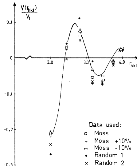
FIG. 4. Least-squares fit of the form V(r_{hkl})/V_1 \sim A \cos(4.911_0 \epsilon r_{hkl} + \phi)/(r_{hkl})^3 , where \epsilon = (e/at.)^{1/3} , to the five sets of pair-interaction ratios obtained from the different sets of \alpha_i data at T/T_c = 1.091 (see Table II). The theoretical prediction for the interaction ratios is drawn as a continuous curve although it is only the values at the lattice sites r_{hkl} which have significance here. The curve is for A = 1.9 , \epsilon = 0.98 , and \phi = -0.7 .
